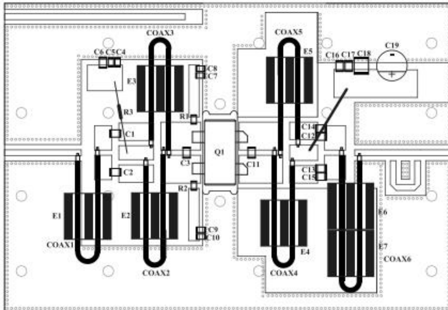
EVB Layout
